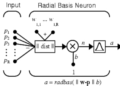
Fig. 1. Radial Basis Function Neural Network.
